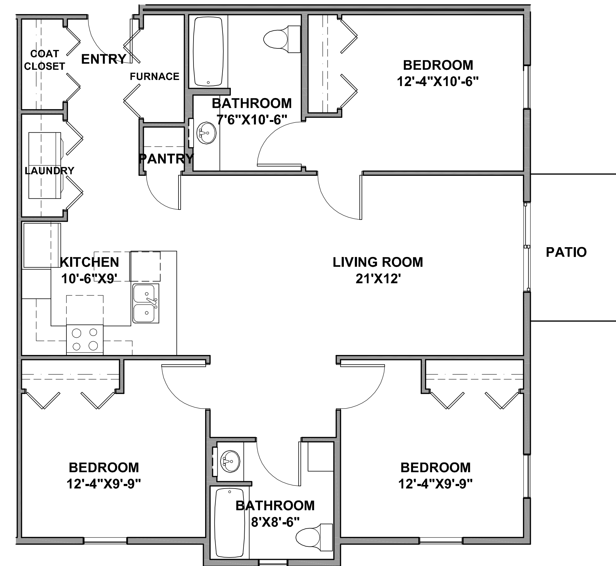
3 ENLARGED PLAN — UNIT C (ADAPTABLE) A2.4 1/4" = 1'0"
